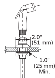
Side Spray (27CI only) Douchette latérale (27CI uniquement) Rociador lateral (solo 27CI)
