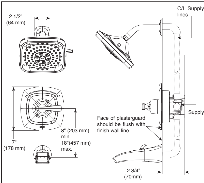
RP52690 ▲ (Showerhead)
